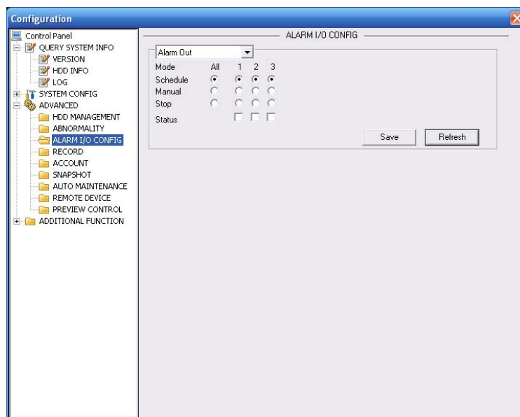
Figure 6-48 Alarm I/O Configuration
